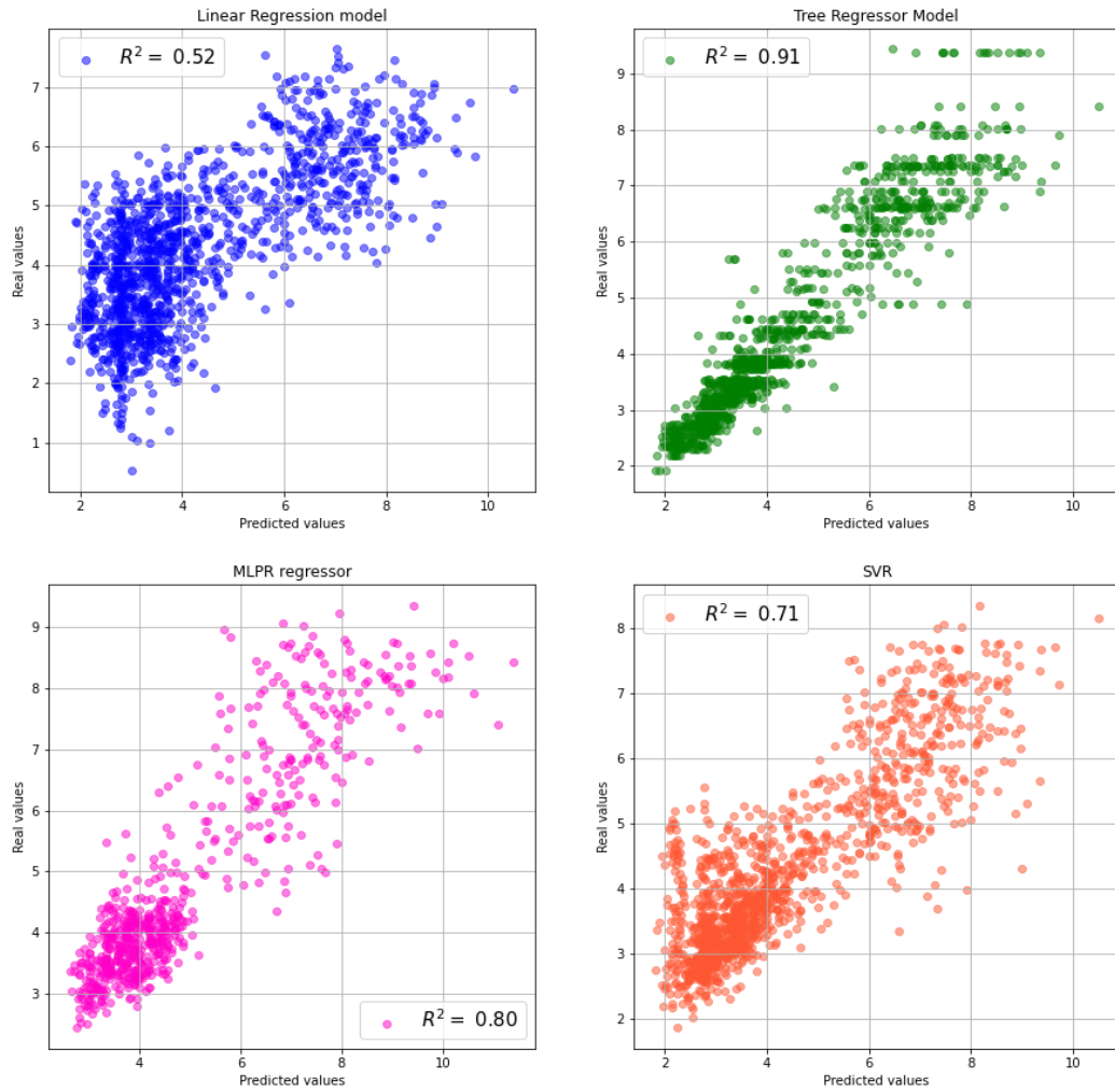
Figure 4: Comparison of real and predicted values.
