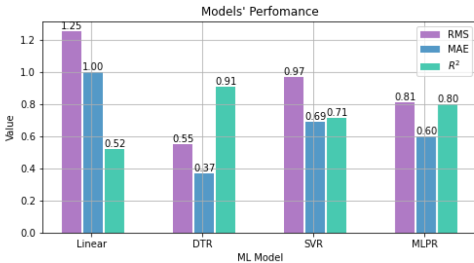
Figure 5: Model Performance Comparison
