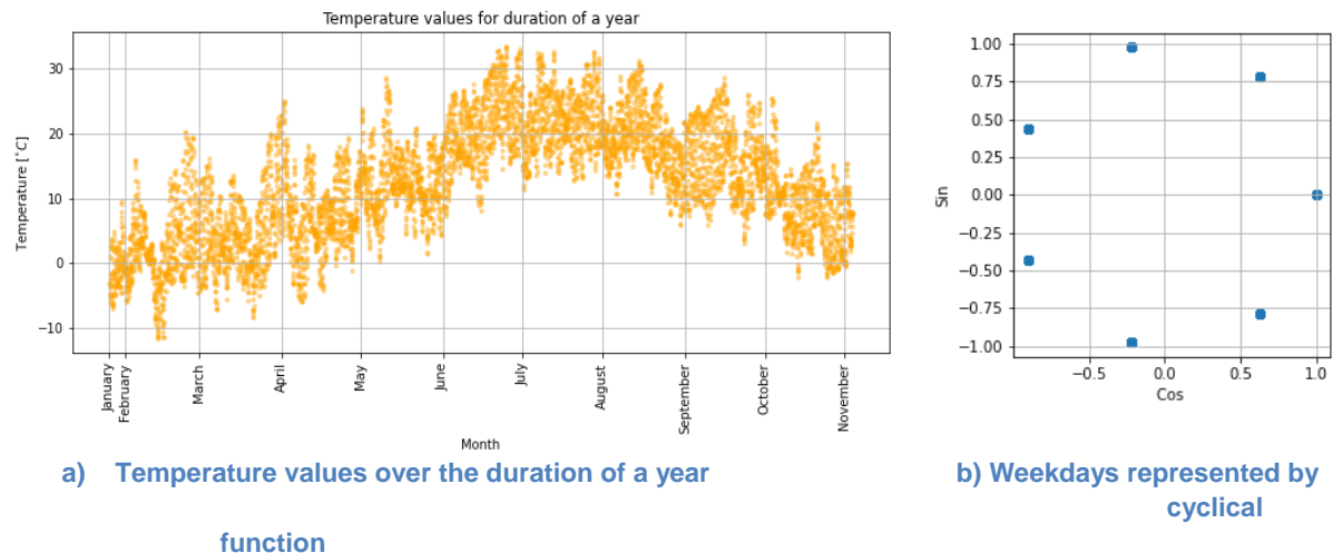
Figure 3: Input features
