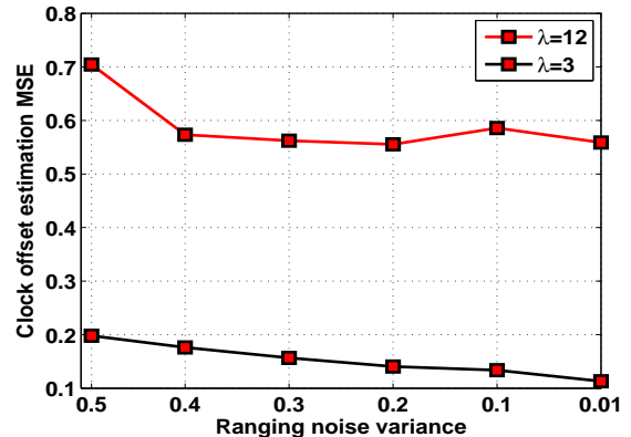
Fig. 2: Clock offset estimation performance
