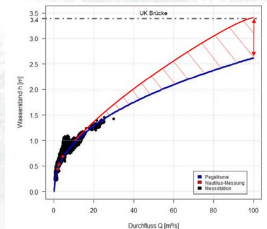
Example of a Rating Curve (Spreitzer, 2014):
