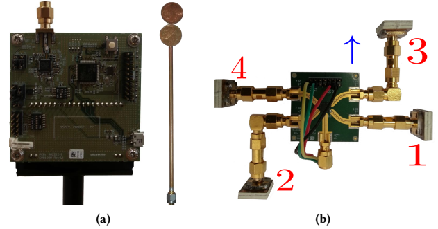
Figure 1: Decawave EVB1000 node with omni-directional antenna (a) and switchable directional antenna system (b) [3].
