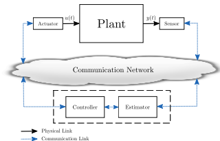
Figure: Networked Control System (NCS)
