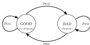
Figure: Gilbert-Elliot network dropout model
