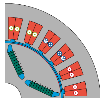
Model of a permanent magnet synchronous motor to be analyzed and optimized.
