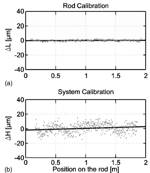
Fig. 8. Calibration results for Trimble rod 13702 determined: (a) by rod calibration; (b) by system calibration in combination with Trimble DiNi12
