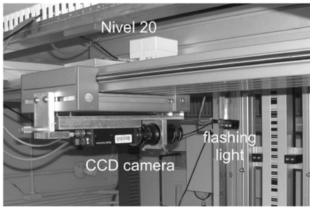
Fig. 3. CCD camera setup as part of SLAC vertical comparator
