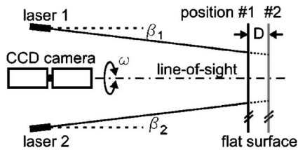
Fig. 6. Top view of setup used for horizontal alignment of CCD camera
