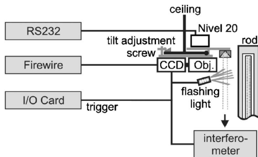
Fig. 4. Schematic overview of CCD camera part of SLAC vertical comparator (for location of CCD section see Fig. 2)
