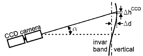
Fig. 5. Effect of tilted camera on height readings (side view)
