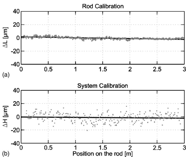
Fig. 7. Calibration results for Leica rod 9960 determined: (a) by rod calibration; (b) by system calibration in combination with Leica DNA03
