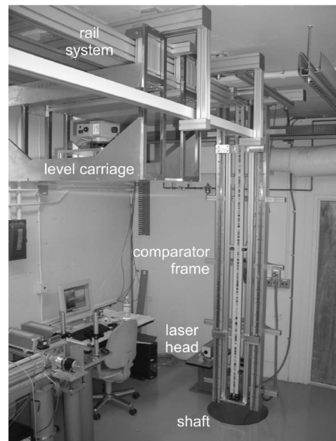
Fig. 2. SLAC vertical comparator
