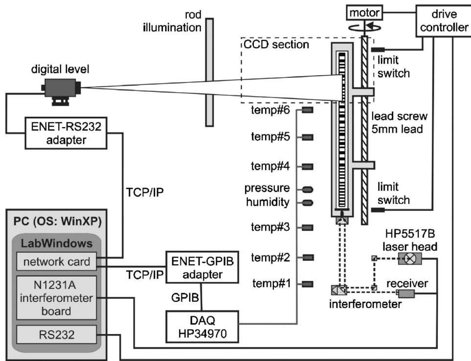
Fig. 1. Block diagram of vertical comparator for system calibration of digital levels
