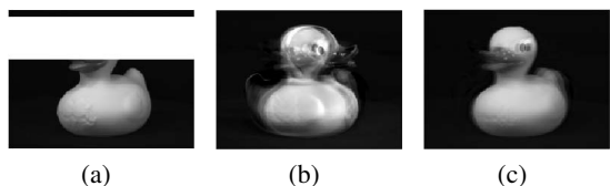
Figure 3: Demonstration of the insensitivity of the robust PCA to occlusions. (a) Occluded image, (b) reconstruction using standard PCA, and (c) reconstruction using the FR-PCA.
