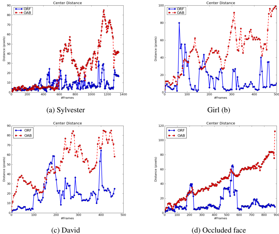
Figure 2. Comparison of ORFs with OAB on four state-of-the-art tracking sequences. As can be seen, our method significantly outperforms boosting on all sequences.
