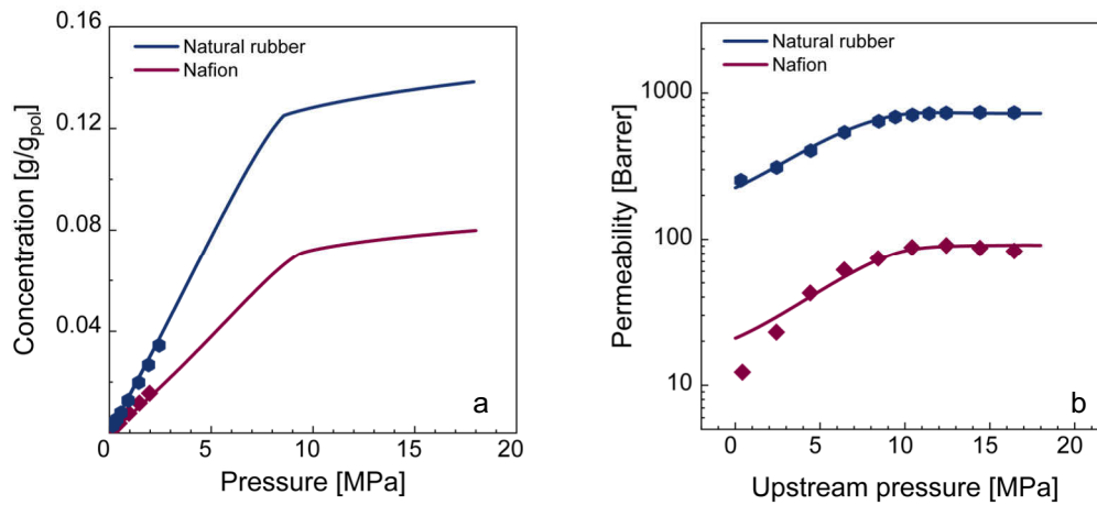
Figure 2, Sorption and permeability of CO 2 in Natural rubber and Nafion. Experimental data are from: (a)[12,13] (b) [14]. Curves are from (a) EoS and (b) ST calculations.
