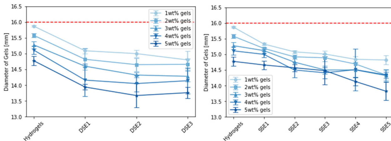
Figure 3: The shrinkage of hydrogels and alcogels in direct solvent exchange (DSE) on the left and step-wise solvent exchange (SSE) on the right, for alginate gels of concentration 1 to 5 wt%.
