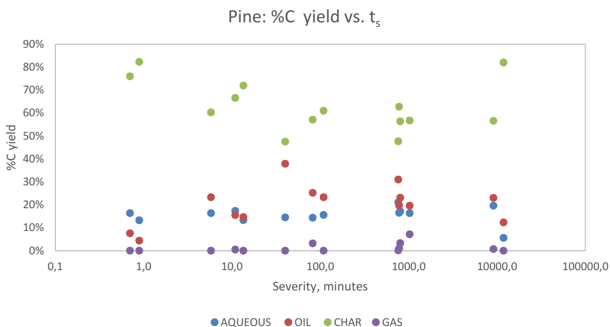
Fig. 1. Carbon yield (%) vs. severity factor for batch experiments with pine
