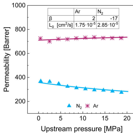
Figure 3, Permeability of \text{N}_2 and Ar in PDMS at 45°C. Experimental data from [14,20]. Curves are from STM calculations.
