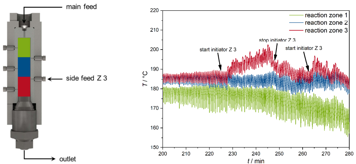
Fig. 3.: Temperature profile of an LDPE-experiment after the start of the initiator feed into the third zone of the multi-zone autoclave.
