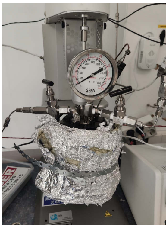
Fig. 2.: Image of the 50 mL reactor
