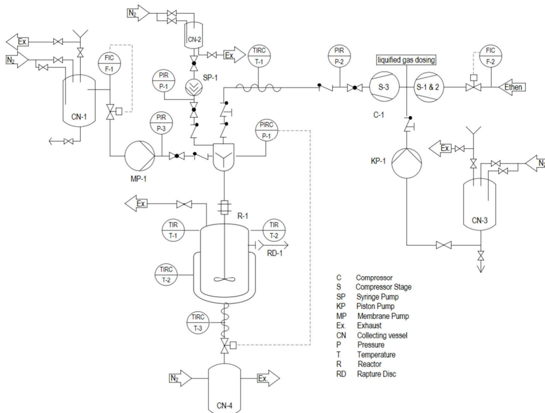
Fig. 1.: Flow diagram of the experimental setup of the continuous high-pressure mini-plant.
