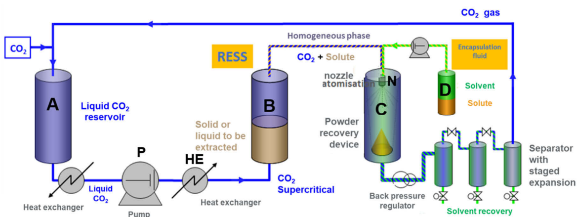
Fig. 2.: Supercritical CO 2 extraction and encapsulation process
