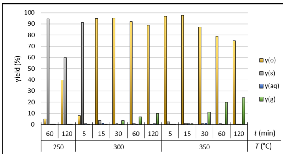
Fig. 1. Yield of oil ( y(o) ), solid ( y(s) ), aqueous ( y(aq) ) and gas ( y(g) ) phase after hydrothermal degradation of PC.
