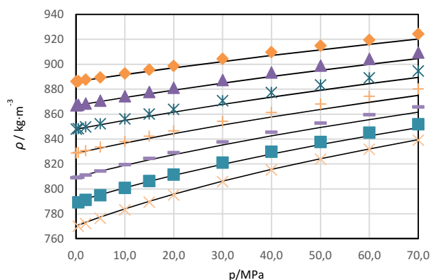
Fig. 1: Experimental density data of toluene (♦ 273.15 K; ▲ 293.15 K; ✱ 313.15 K; + 333.15 K; - 353.15 K; ■ 373.15 K; x 393.15 K; - \rho /Tamman-Tait).
