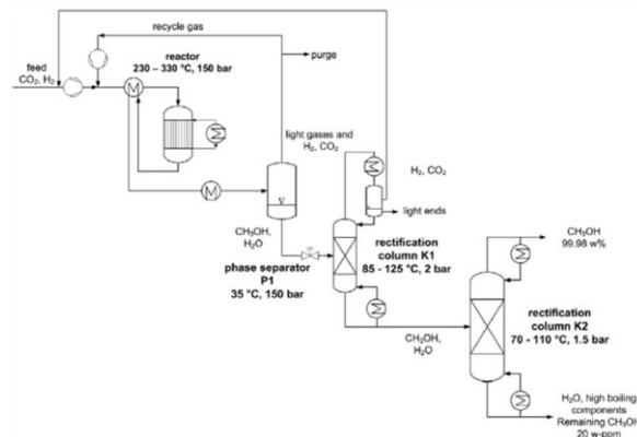
Fig. 3: Process concept proposal for CH 3 OH synthesis [5]
