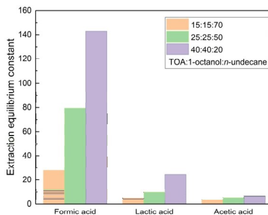
Fig. 7: Equilibrium constant for formic-, acetic - and lactic acid in dependency of the organic phase
