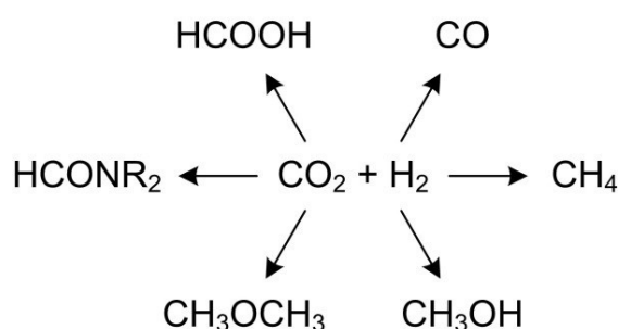
Fig. 1: Different possible products of \text{CO}_2 hydrogenation The methane ( \text{CH}_4 ) production, also known as Sabatier reaction, is applied for syngas production and formation of compressed natural gas. Carbon monoxide ( \text{CO} ) is an important substance for methanol ( \text{CH}_3\text{OH} ) and long
