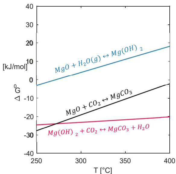
Fig. 1: Gibbs free enthalpy \Delta G^0 for Mg reactions with CO 2 and water
