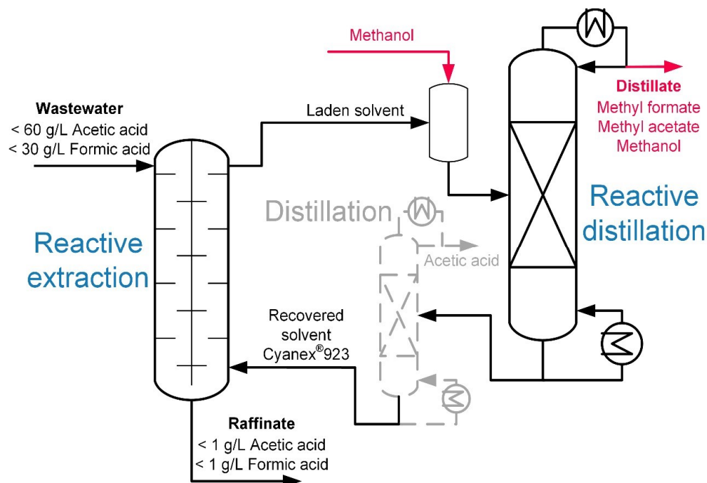
Fig. 1: Reactive separation concept for acid recovery from wastewater. Combination of reactive extraction for acid removal from the effluent and reactive distillation for solvent regeneration
