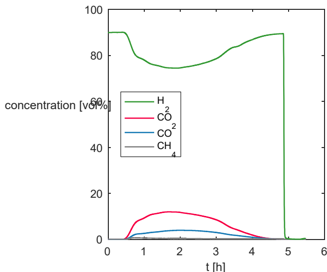
Fig. 3: Composition of the gas product during the experiment with 420°C, H 2 :N 2 =9:1, particle size 1–2 mm and 132 g iron ore
