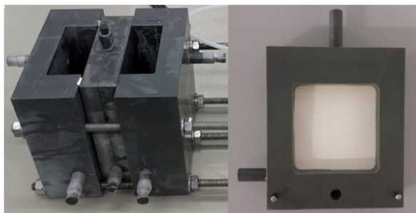
Fig. 5: Supported liquid membrane configuration
