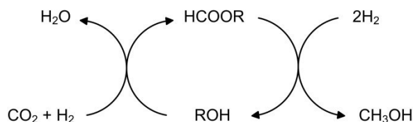
Fig. 2: Reaction mechanism for a low temperature route presented by Liu et al. [4]
