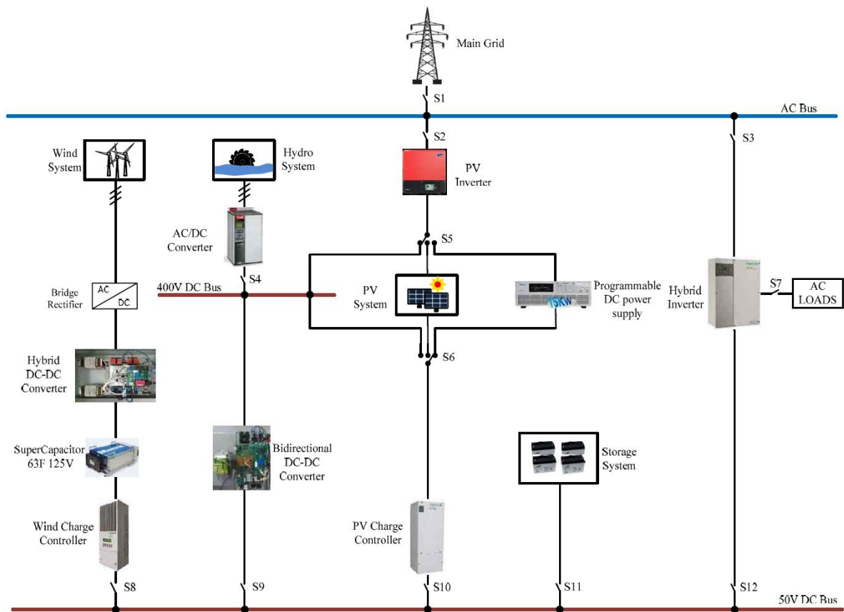
UPT microgrid topology
