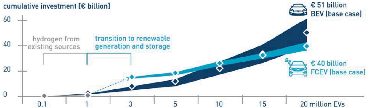
Figure 2: Comparison of the cumulative investment of supply infrastructures.
