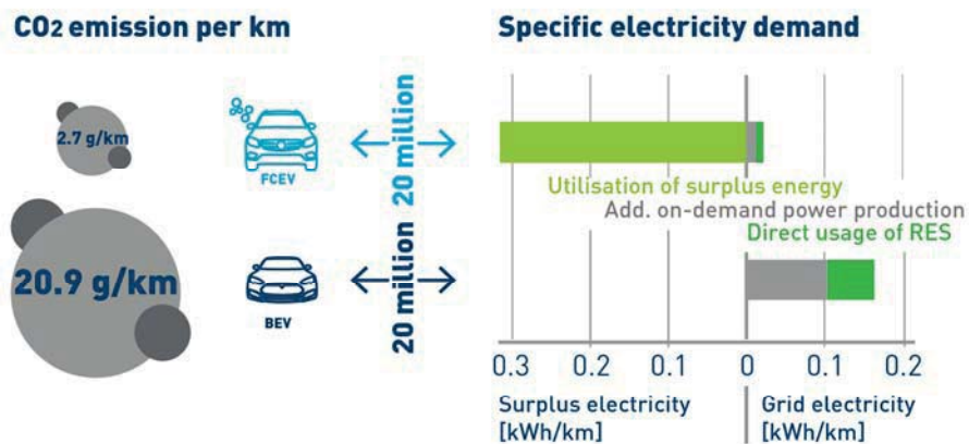
Figure 3: Comparison of specific energy demand and CO 2 emissions.
