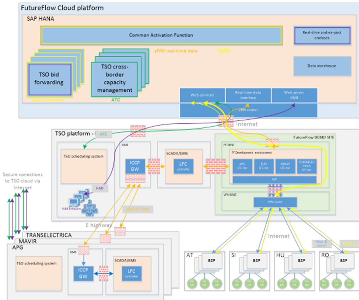
Figure 1: The FutureFlow DEMO Site System Architecture [6]
